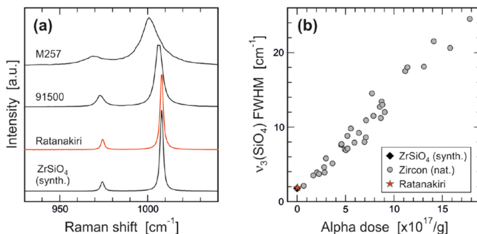
Fig. 2. (a) Raman spectrum of the Ratanakiri zircon in comparison with reference samples, including synthetic \text{ZrSiO}_4 , zircon 91500 (Wiedenbeck et al. 2004; mildly radiation-damaged) and M257 (Nasdala et al. 2008; moderately radiation-damaged). (b) Plot of the width of the main Raman band near 1000 \text{ cm}^{-1} versus alpha dose (from Nasdala et al. 2004, modified). Note that spectral parameters of the Ratanakiri zircon are indistinguishable from those of synthetic \text{ZrSiO}_4 , indicating that the Ratanakiri zircon has accumulated extremely low amounts of radiation damage.
